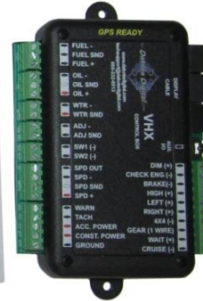
Control Box
