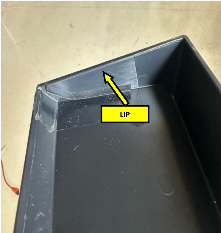
2. Position the lip (see detail) of the new quarter splitter over the ledge of the rear bumper cover, as shown in the view.
