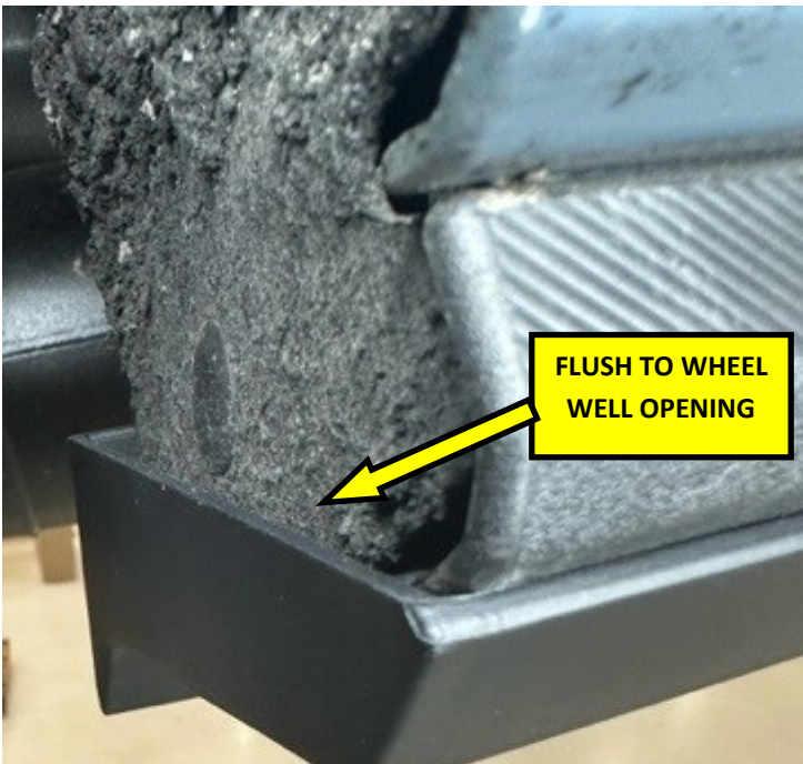
4. Ensure that the flat of the quarter splitter is tight to the rear of the lower wheel well opening.
