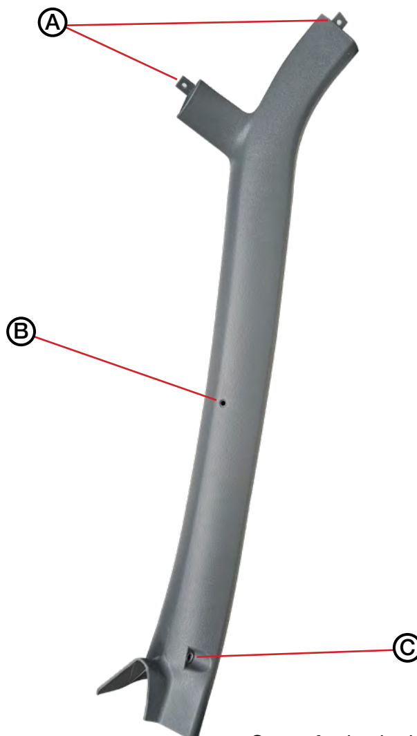
(C) 11/16" Phillips Oval Head SEMS Screws (2)
