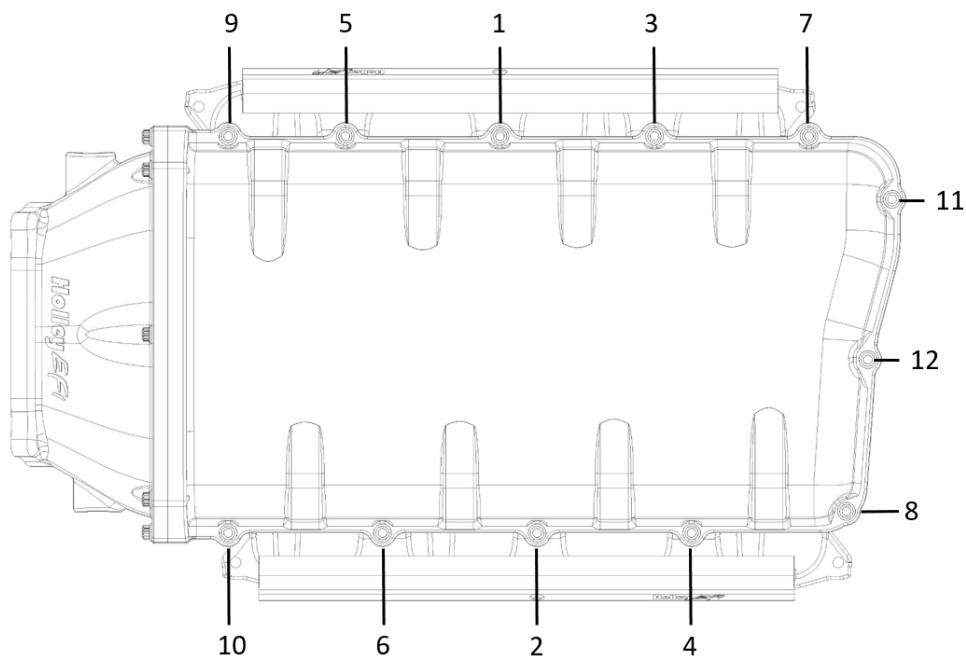
Plenum Top Torque Sequence for 300-911, 300-912
