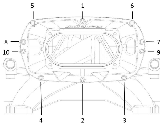
Throttle Body Flange Torque Sequence
