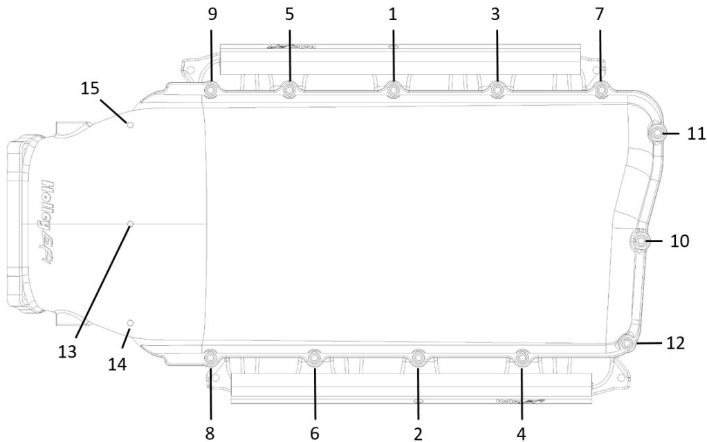
Plenum Top Torque Sequence for 300-910
