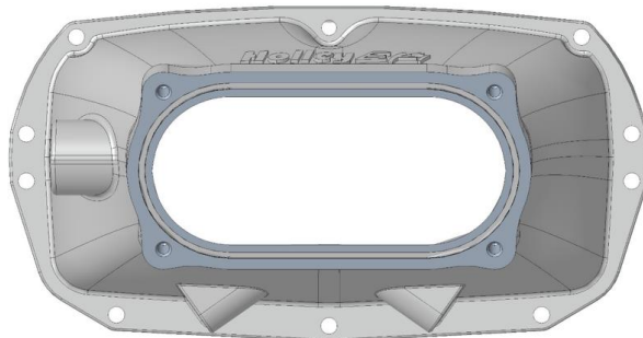
300-911 and 300-924 are designed to work with Ford GT500 (2007-2014) type throttles – throttle opening is 150mm x 66mm
