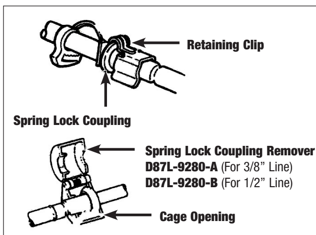
Figure 2 - Disconnecting Fuel Lines
