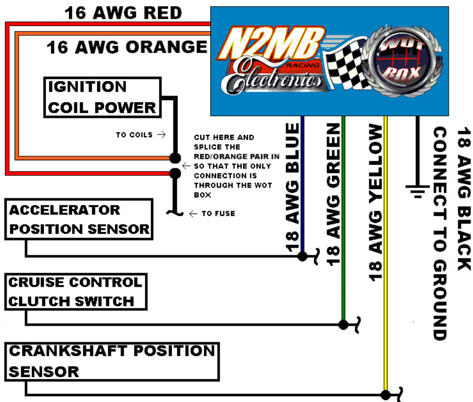
Figure I: Installation schematic
