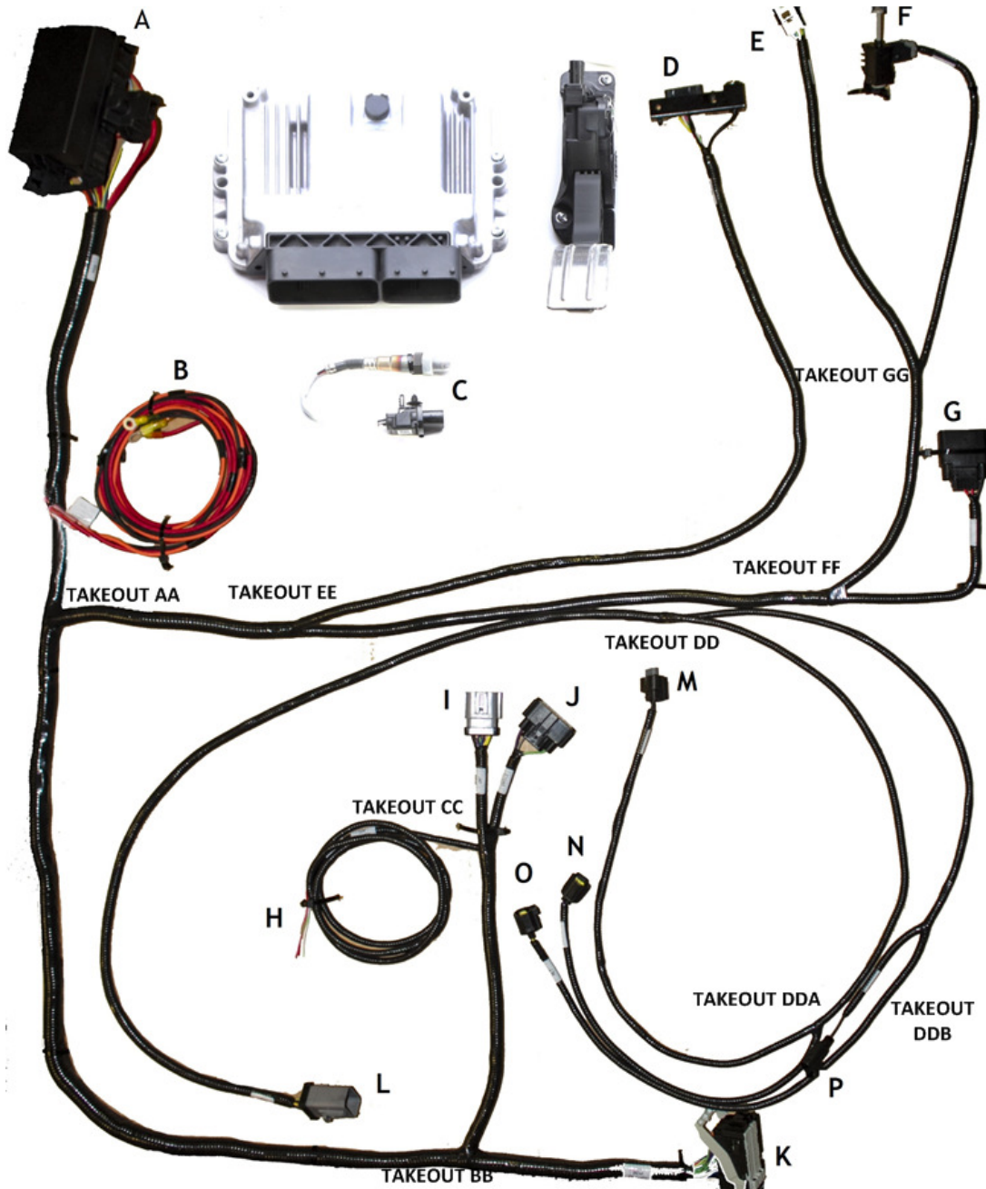
Figure 1 - Controls Pack Wiring Harness Components
