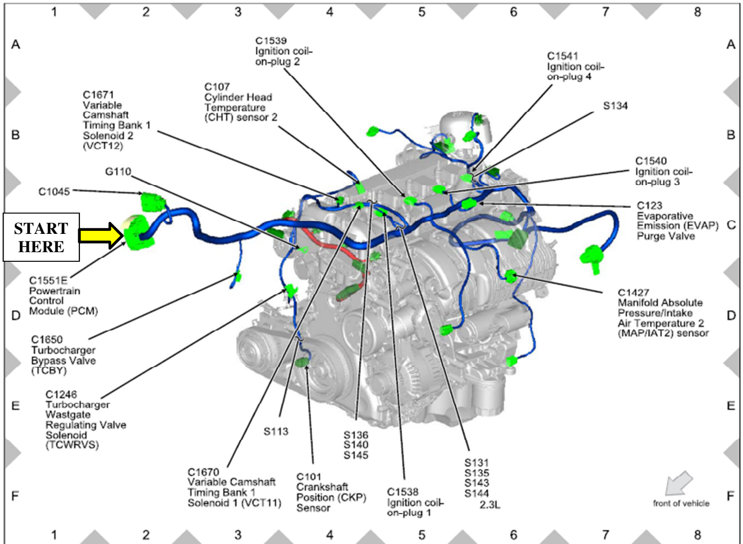
Figure 3 – Front View of Engine.
